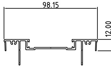
Setting Receiving Track RST-64/19
