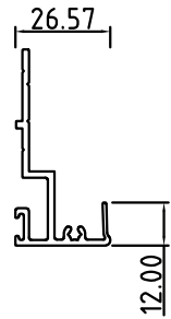
Setting Capping RST-64/17
