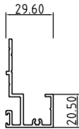
Supreme Cavity Capping SCS-64/17
