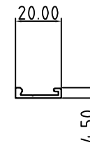
Pelmet Adaptor SCP-28
