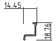
10mm Plaster Board Adaptor DPS-07
