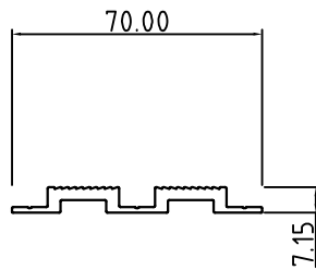
Supreme Carcass Brace SCB-23
