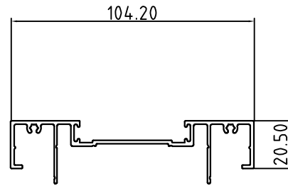
Supreme Receiving Track SCS-64/19
