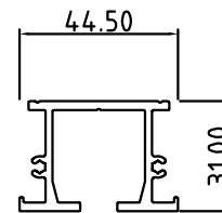
Supreme Cavity Slider Head SCS-76/38
