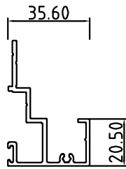
Supreme Cavity Capping SCS-76/17
