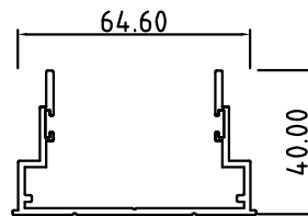
Supreme Receiving Track SCS-76/19
