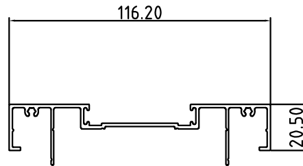
Supreme Receiving Track SCS-76/19
