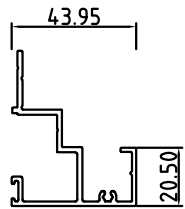
Supreme Cavity Capping SCS-92/17
