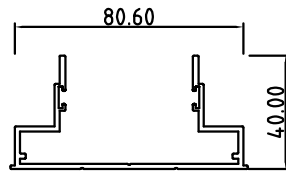
Supreme Carcass Channel SCS-92/34
